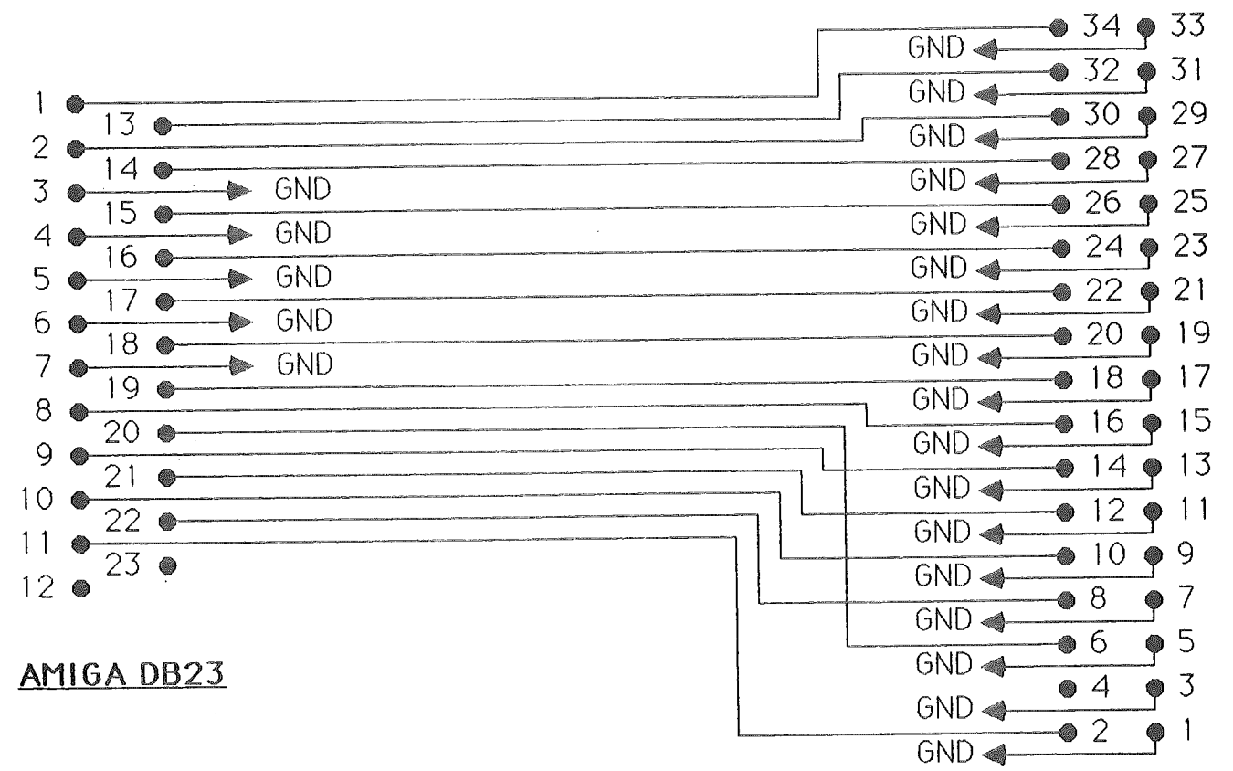
Fig. 2: Cable for modified drives
