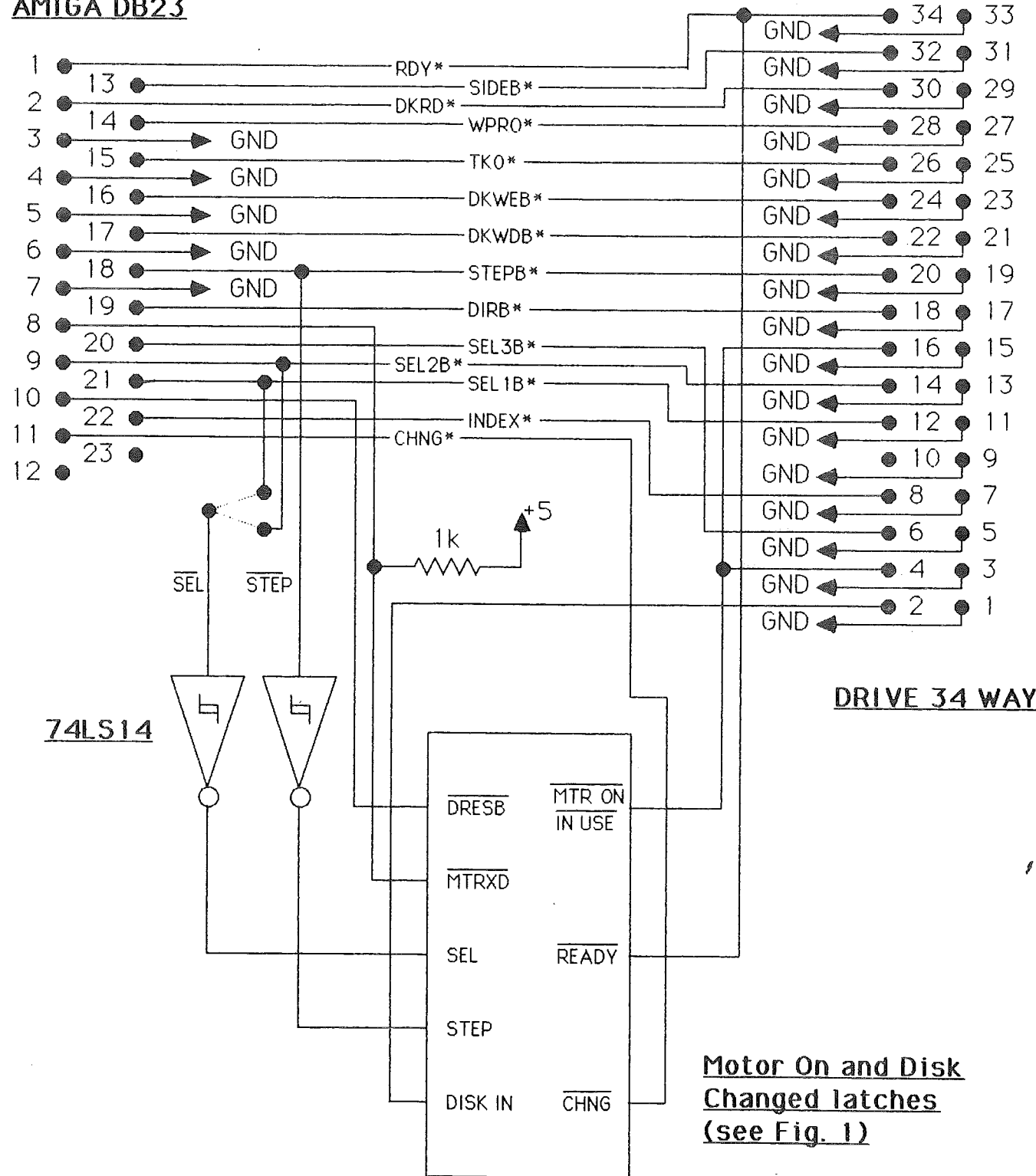
Fig. 5: Adaptor for minimally modified drive
