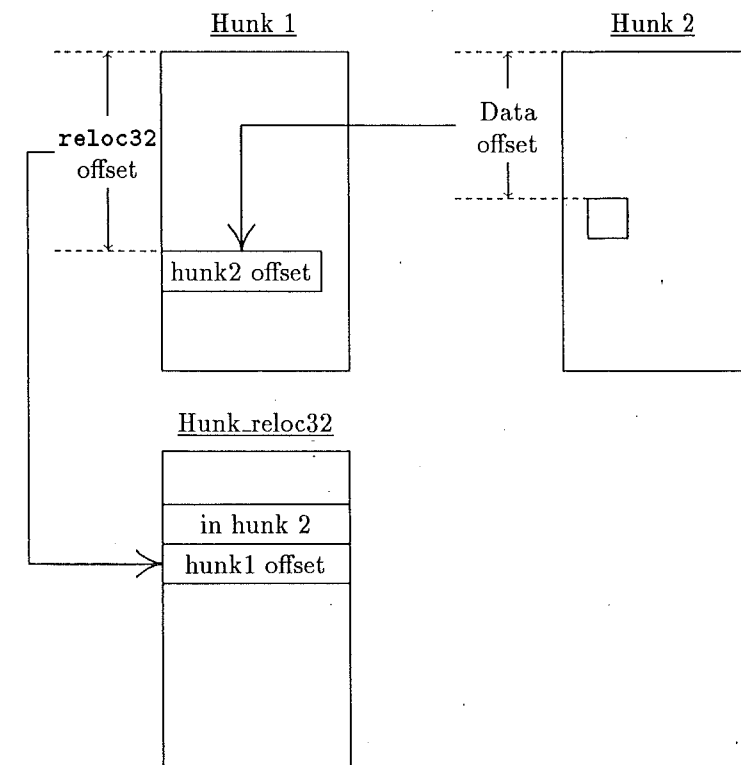
Fig. 1—The reloc32 Process
