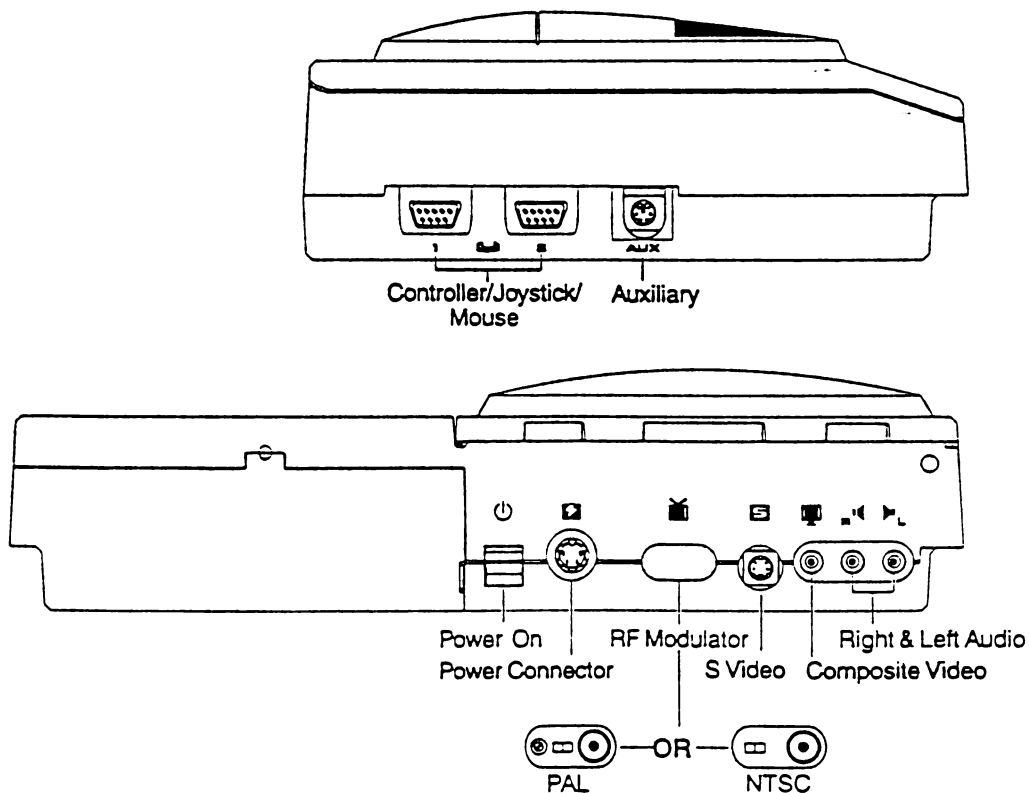
Figure 1-2. Side and Rear Panels
