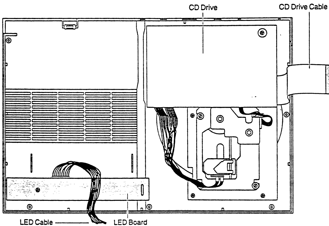
Figure 2-1. CD Player and LED Board Location and Cables
